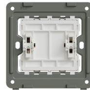
D1003 2 Gang 1 Way Switch 10A 250V~50/60Hz 86mm*86mm
