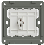
D1001 1 Gang 1 Way Switch 10A 250V~50/60Hz 86mm*86mm
