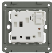
D1011 UK Socket with Double pole Switch 13A 250V~50/60Hz 86mm*86mm
