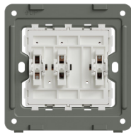
D1005 3 Gang 1 Way Switch 10A 250V~50/60Hz 86mm*86mm
