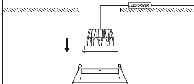
3 Snap the LED cup into the outer ring
