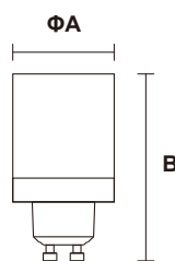
GU10 TO E27 Item Code:NR-GU10-E27
