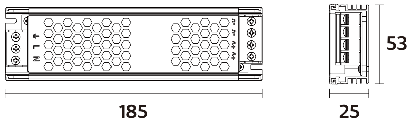
NR-PS102-24V-150W
