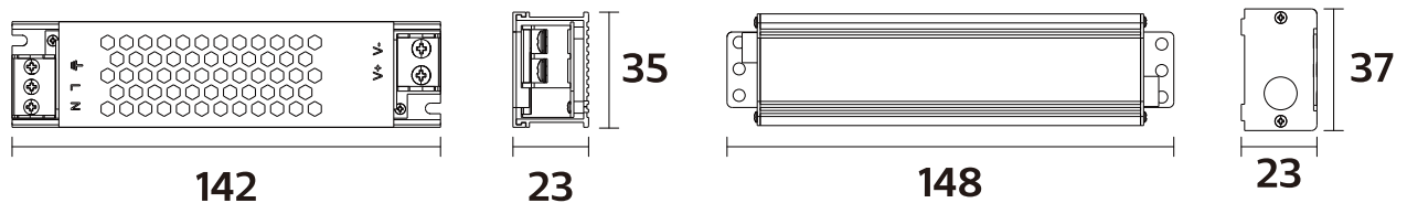
NR-PS102-24V-60W
