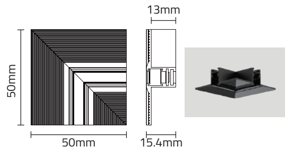
Model No:NR-ST-550TRA-L-Ceiling
