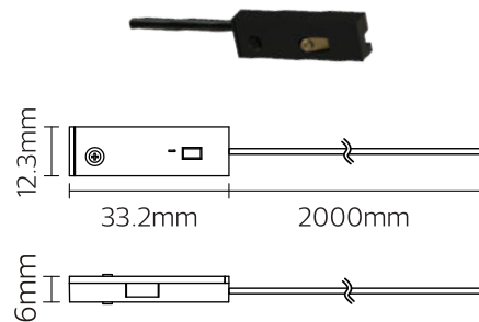
Model No:NR-ST-553TRA-POWER-200CM
