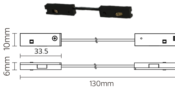
Model No:NR-ST-553TRA-L-CONNECT
