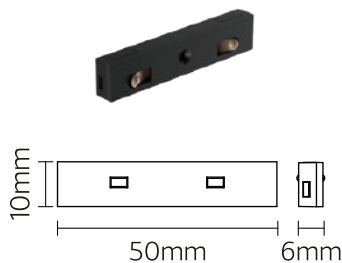
Model No:NR-ST-553TRA-CONNECT
