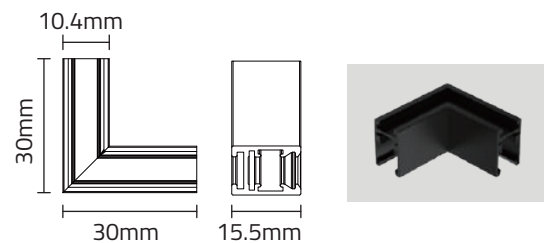
Model No:NR-ST-552TRA-L-Ceiling
