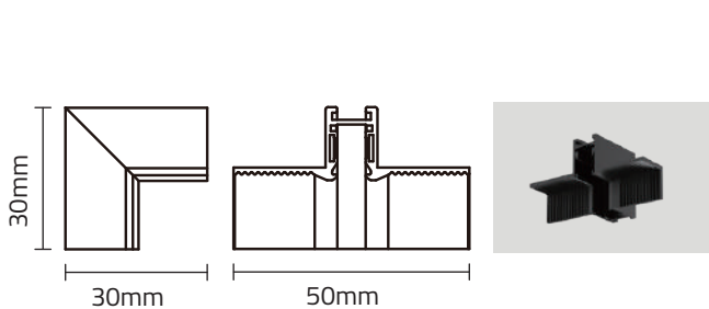
Model No:NR-ST-550TRA-L
