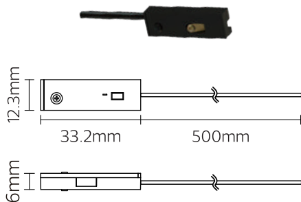
Model No:NR-ST-553TRA-POWER-50CM
