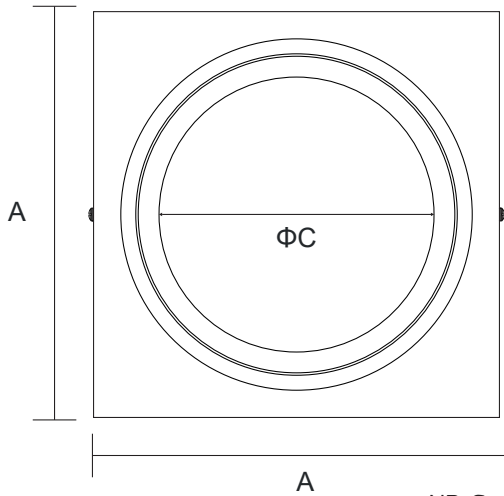
NR-Surface-200-SQ
