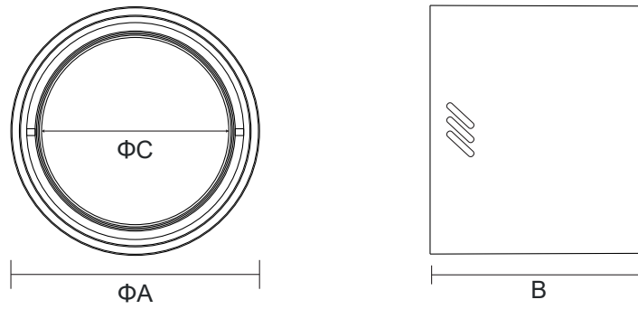
NR-Surface-AR111
