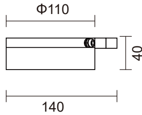
NR-TYD-GX53-100-B
